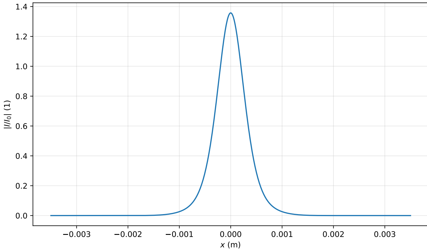
Intensity profile I(x, y = 0, z = 1.513m)/I_0 , P_{in}=0.8P_{cr} , artificial time
